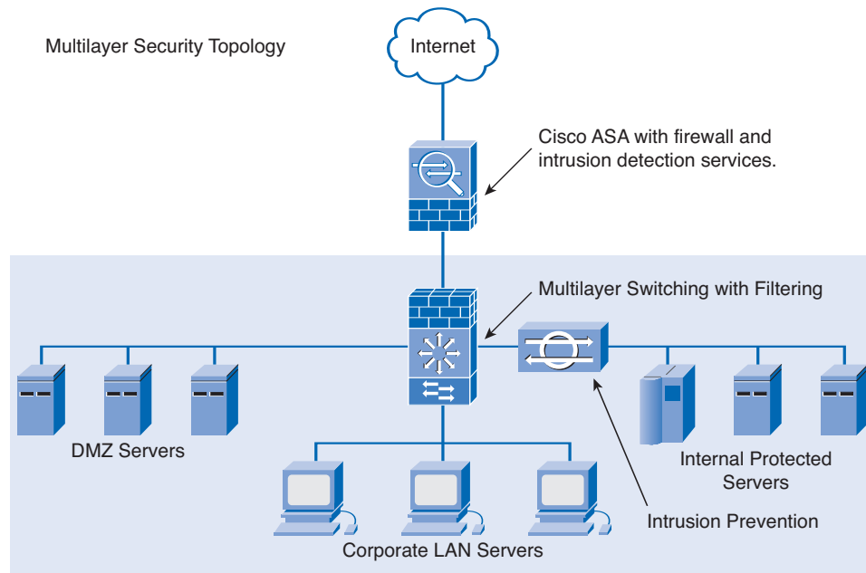
Figure 1-25 Multilayer Security
