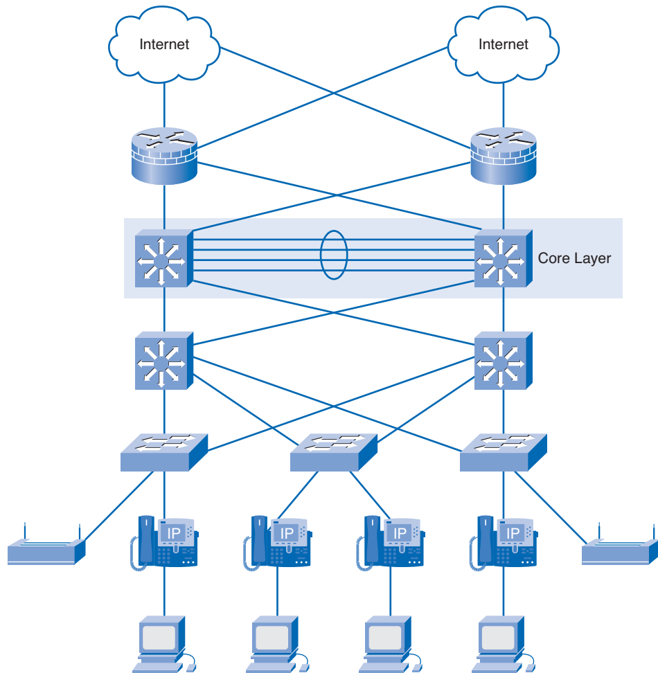
Figure 1-7 Core Layer
