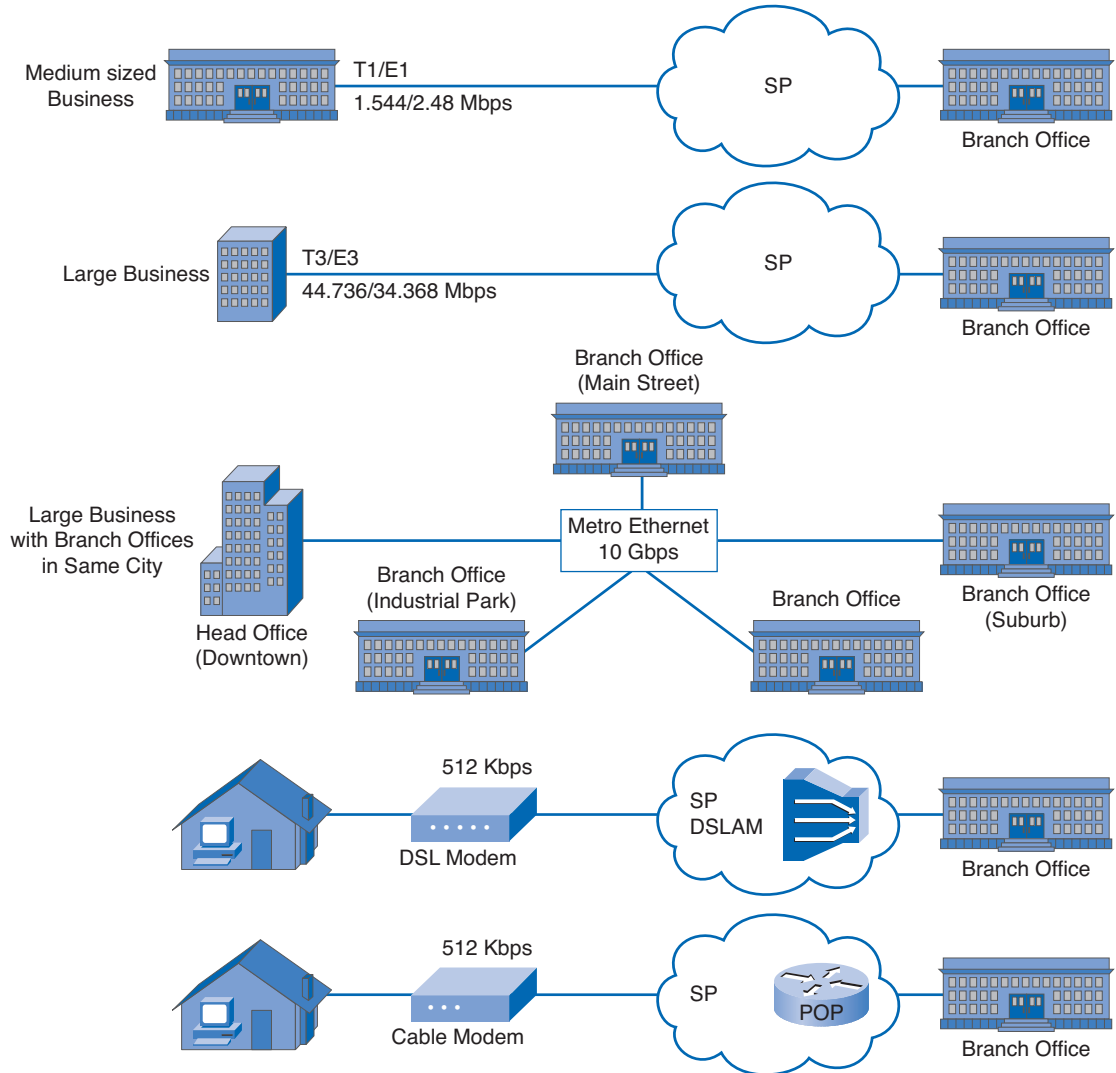
Figure 1-31 WAN Technologies
