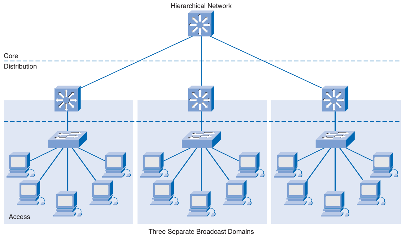
Figure 1-2 Hierarchical Network
